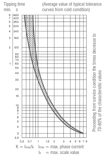
With two-pole load
