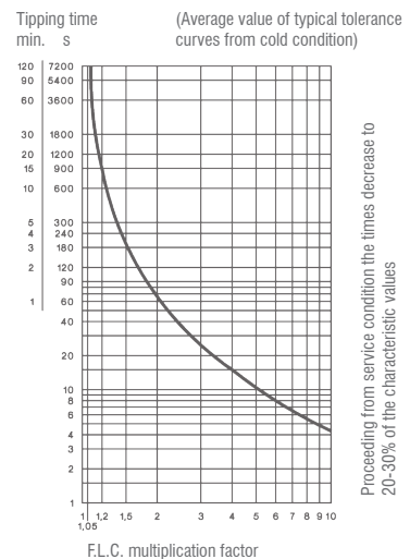
MCOR-7 with three-phase load
