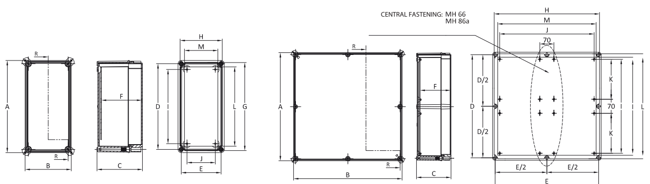
Box dimensions (mm)
